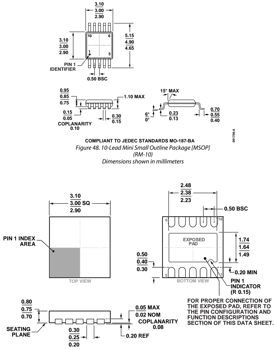
Figure 49. 10-Lead Frame Chip Scale Package [LFCSF_WD] 3 mm × 3 mm Body, Very Thin, Dual Lead (CP-10-9) Dimensions shown in millimeters
