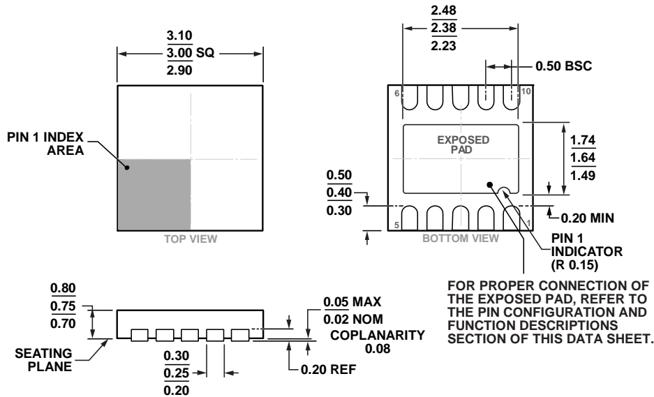
Figure 49. 10-Lead Frame Chip Scale Package [LFCSP_WD] 3 mm x 3 mm Body, Very Thin, Dual Lead (CP-10-9) Dimensions shown in millimeters
