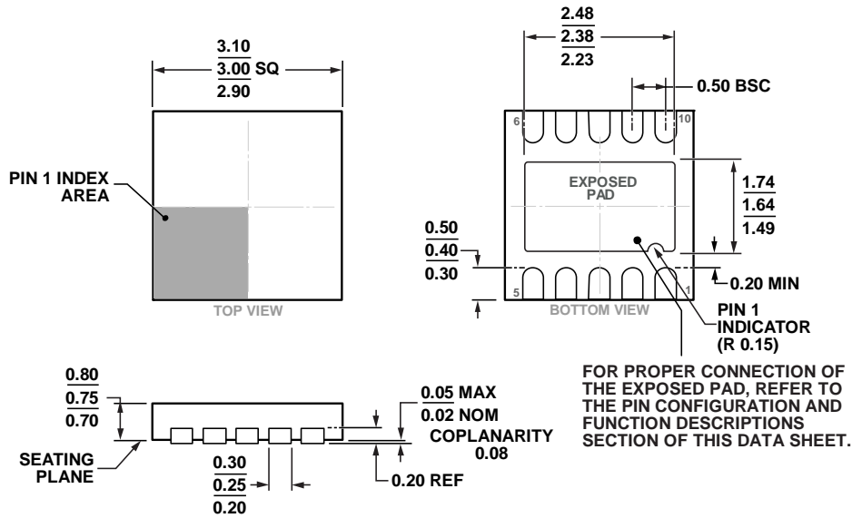
Figure 49. 10-Lead Frame Chip Scale Package [LFCSF_WD] 3 mm × 3 mm Body, Very Thin, Dual Lead (CP-10-9) Dimensions shown in millimeters
