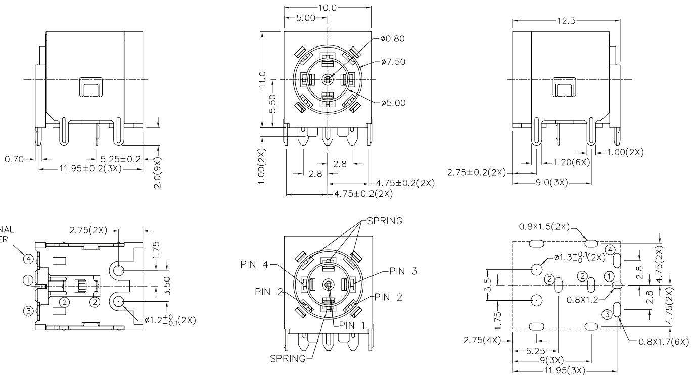
Recommended PCB Layout Top View
