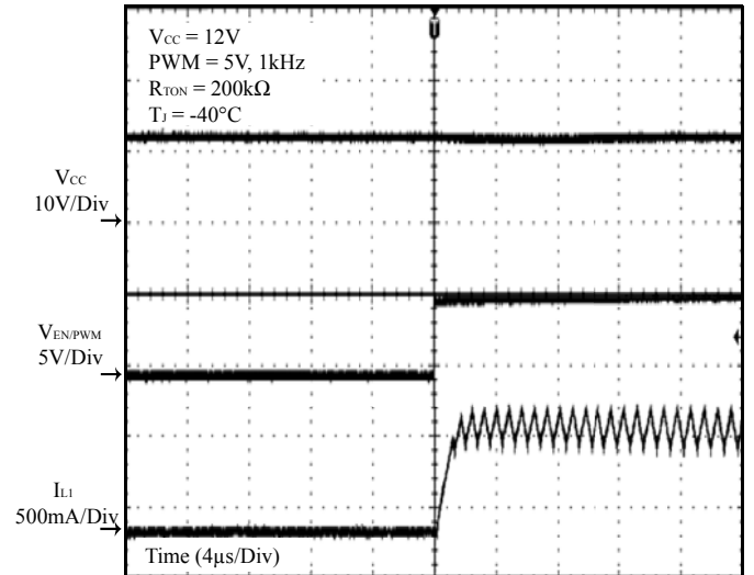
Figure 21 PWM On
