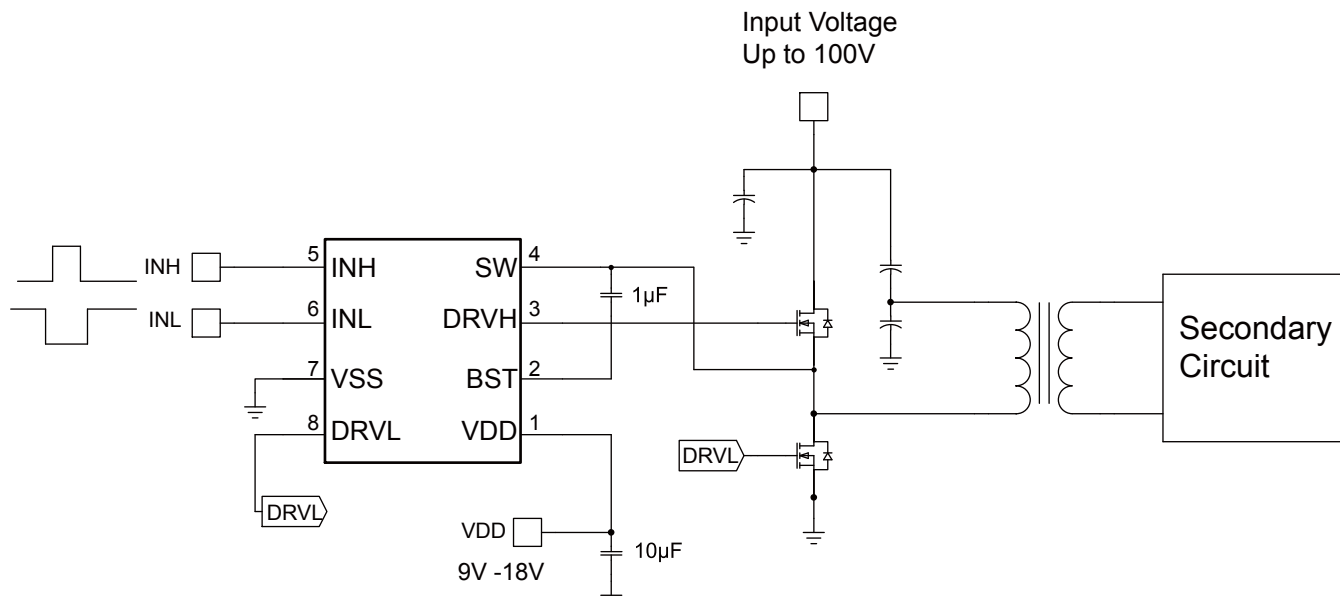
Figure 4: Half-Bridge Converter
