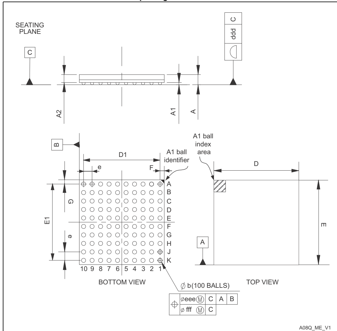
Figure 87. TFBGA100, 8 × 8 × 0.8 mm thin fine-pitch ball grid array package outline
