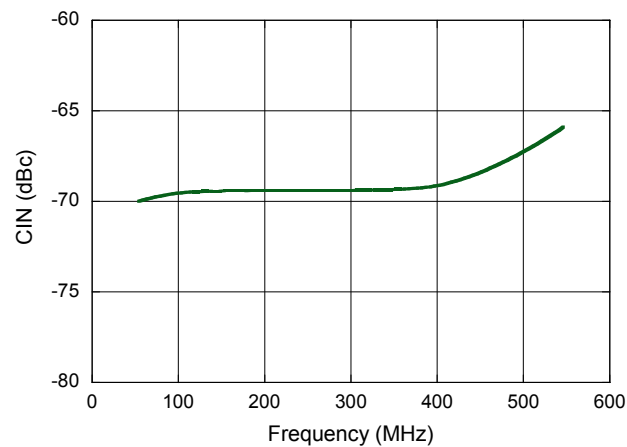
Carrier to Intermodulation Noise
