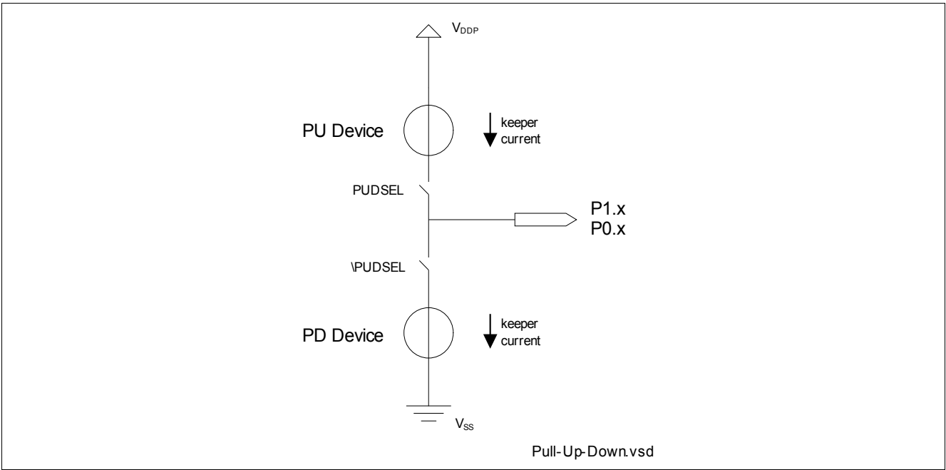
Figure 37 Pull-Up/Down Device
