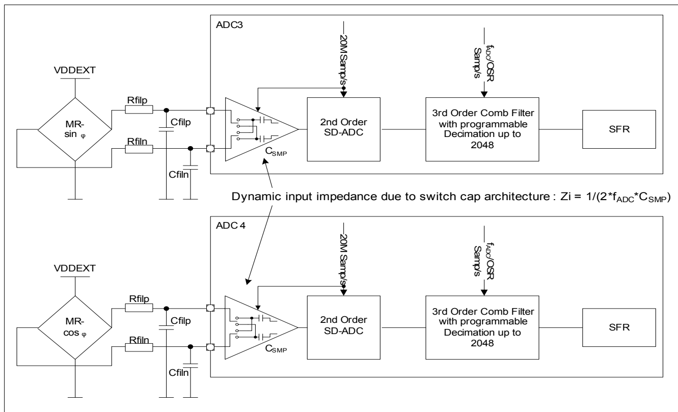
Figure 29 Application of Integrated Sigma Delta ADCs
