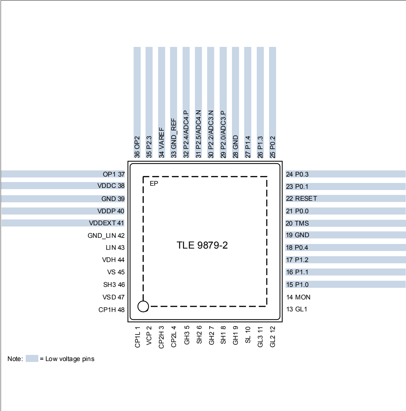
Figure 3 Device Pinout
