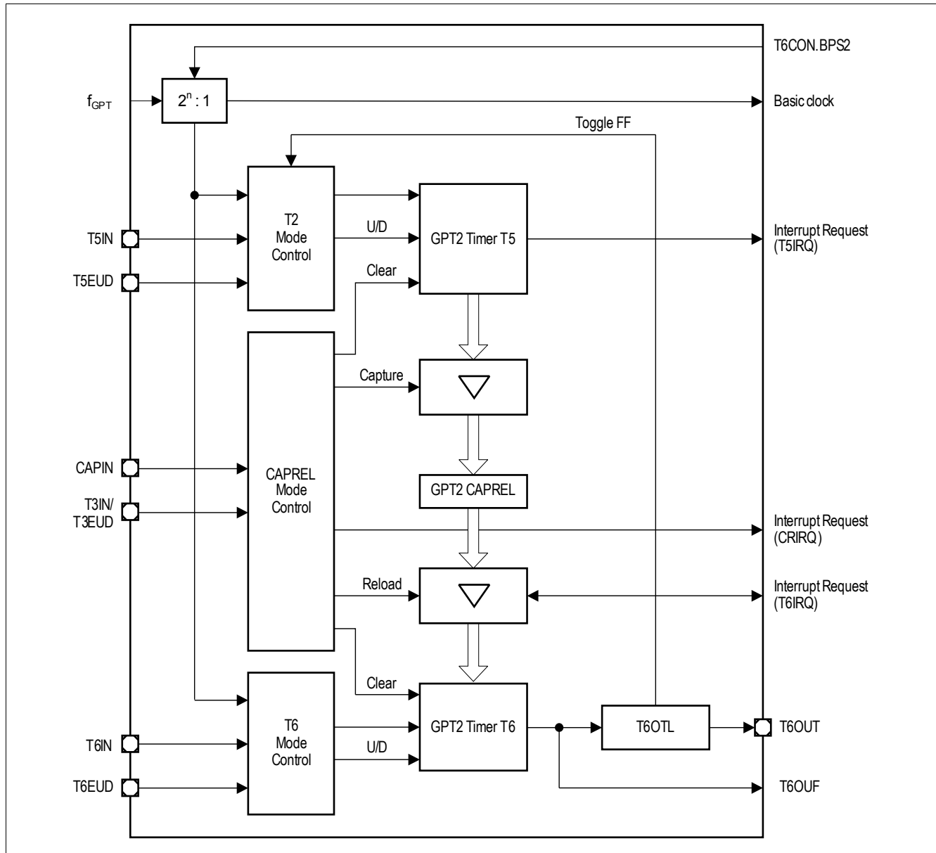
Figure 20 GPT2 Block Diagram ( n = 1 \dots 4 )
