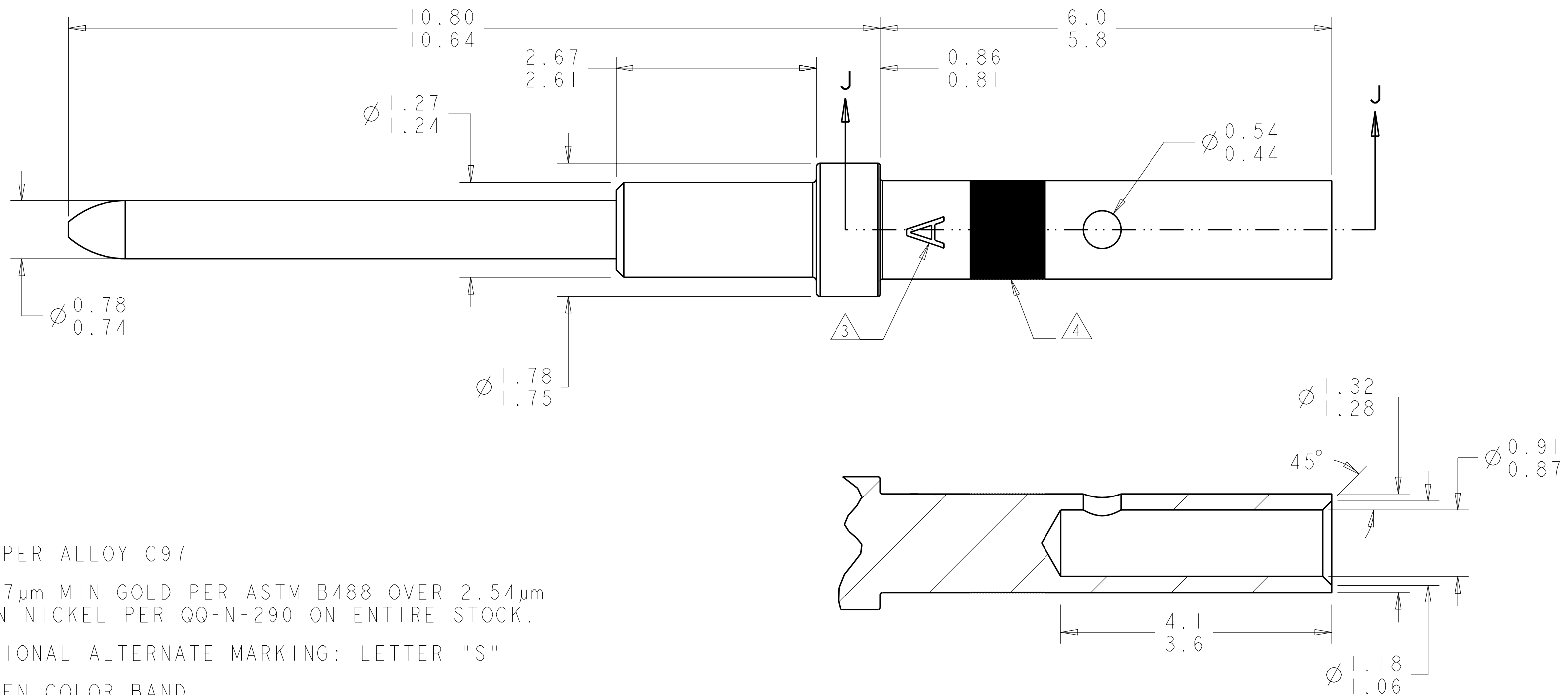
SECTION J-J
