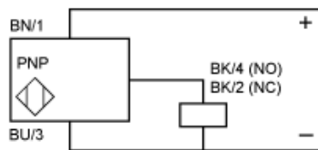
PNP 3-wire
