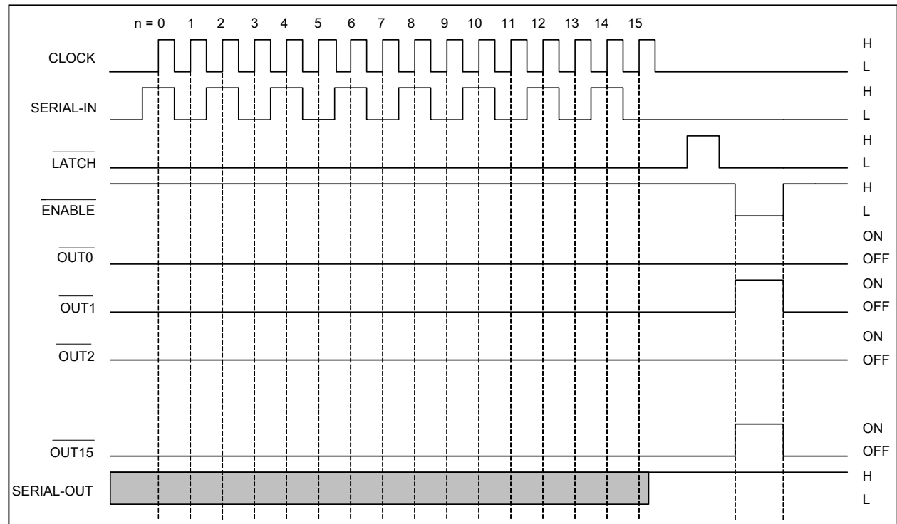
Figure 3 Timing Diagram
