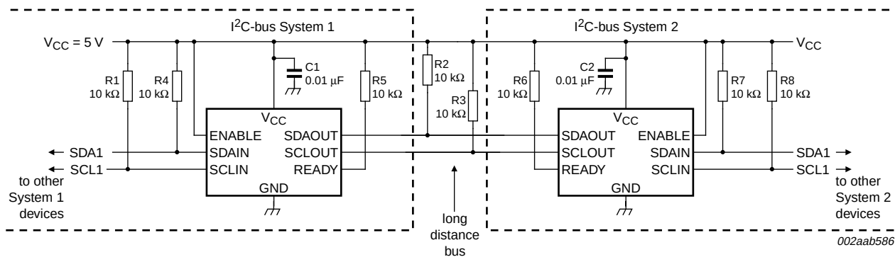
Fig 9. Repeater/bus extender application using the PCA9511A
