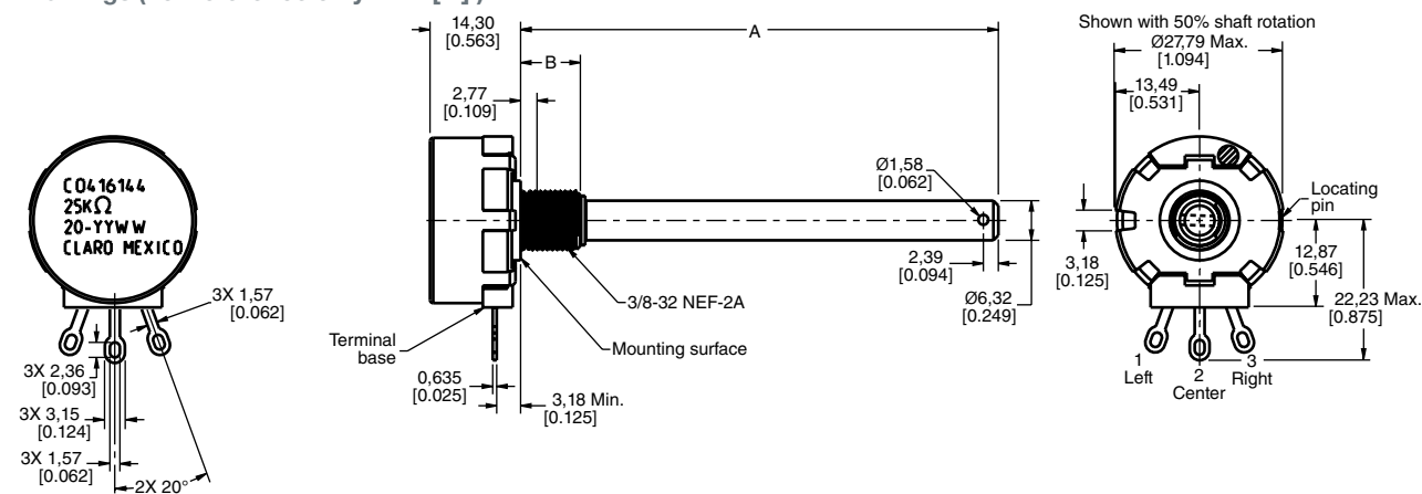
Dimensional Drawings (For reference only: mm [in].)
