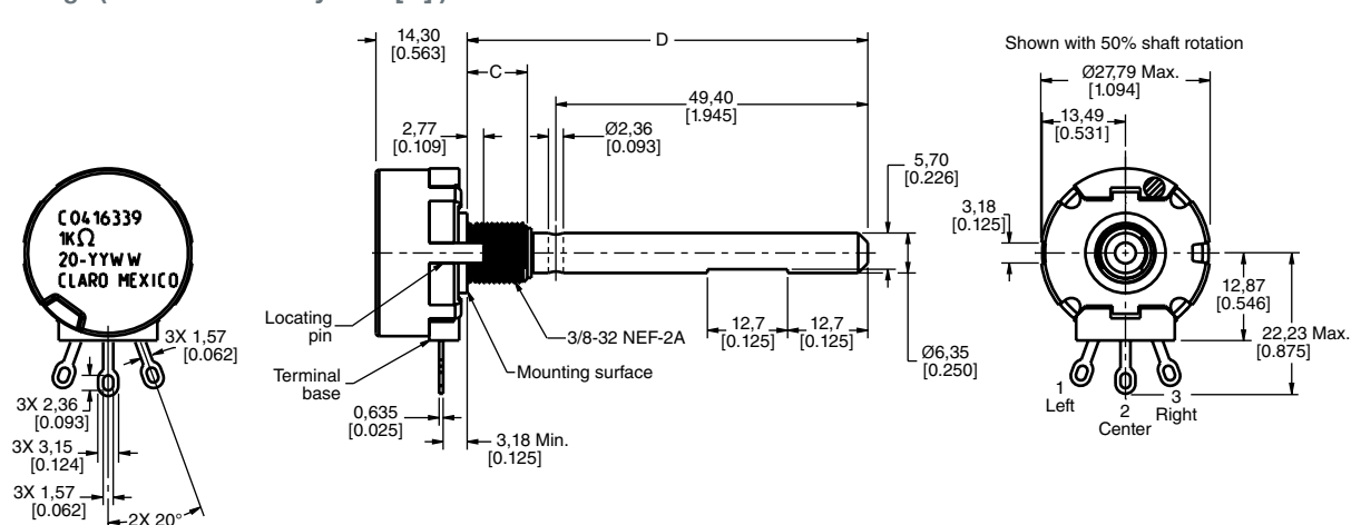
Dimensional Drawings (For reference only: mm [in].)
