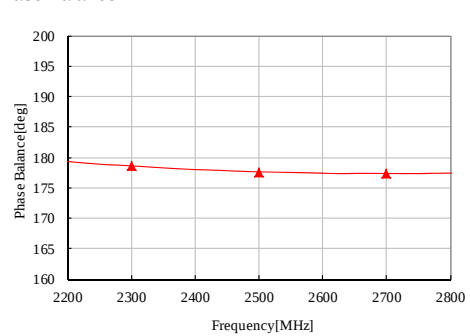
Phase Balance
