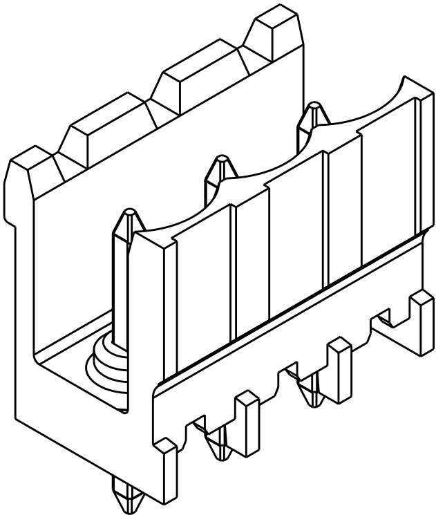
1776138-3 AS SHOWN
