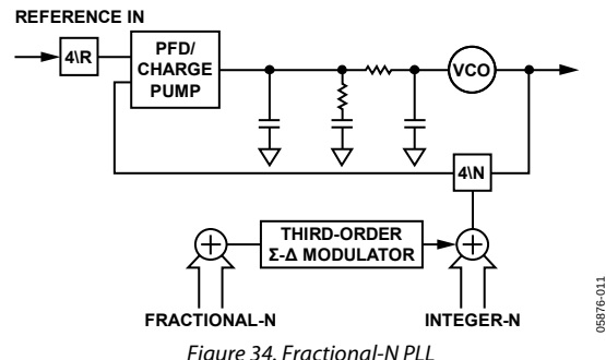
Figure 34. Fractional-N PLL
