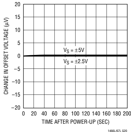
Input Offset Drift vs Time
