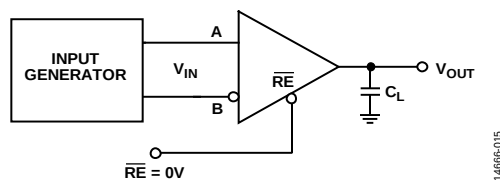
Figure 42. Receiver Propagation Delay/Skew
