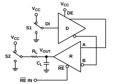
Figure 43. Receiver Enable/Disable from Shutdown
