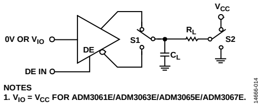
Figure 41. Driver Enable/Disable
