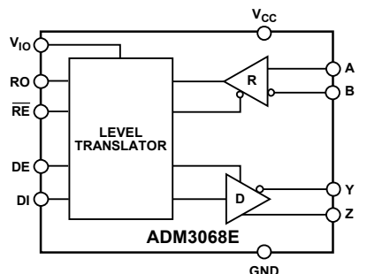
Figure 4. ADM3068E Functional Block Diagram
