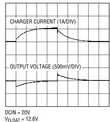
1A Load Step (Battery Present)
