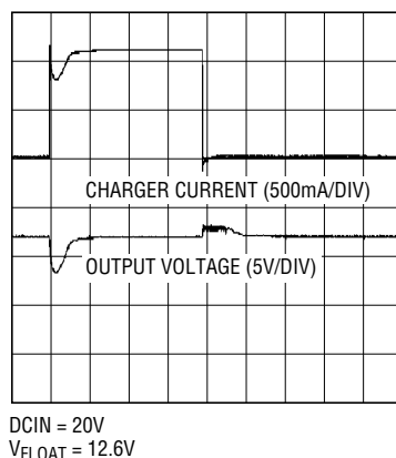
1A Load Step (Battery Not Present)
