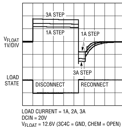
Disconnect/Reconnect Battery (Load Dump)
