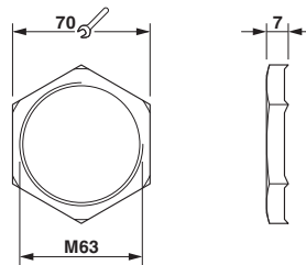
Dimensional drawing
