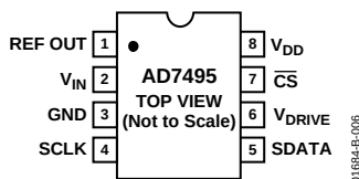
Figure 6. AD7495 SOIC/MSOP Pin Configuration
