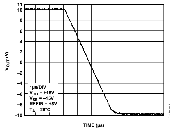
Figure 28. Settling Time
