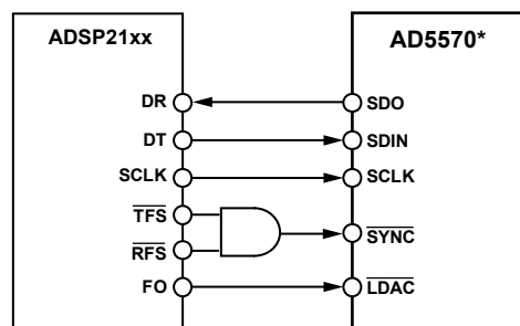
Figure 44. AD5570 to ADSP21xx Interface
