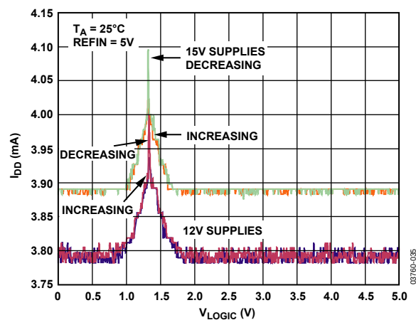
Figure 27. Supply Current vs. Logic Input Current for SCLK, \overline{SYNC} , SDIN, and \overline{LDAC} Increasing and Decreasing
