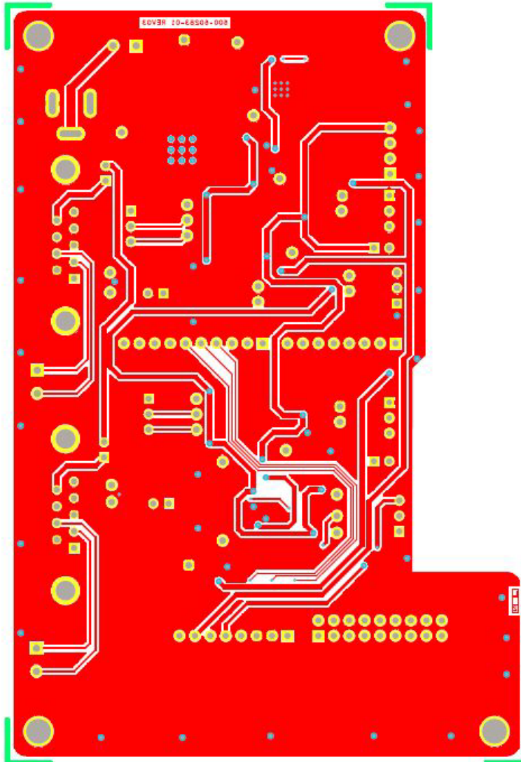
Figure A-6. CY8CKIT-026 Secondary Side
