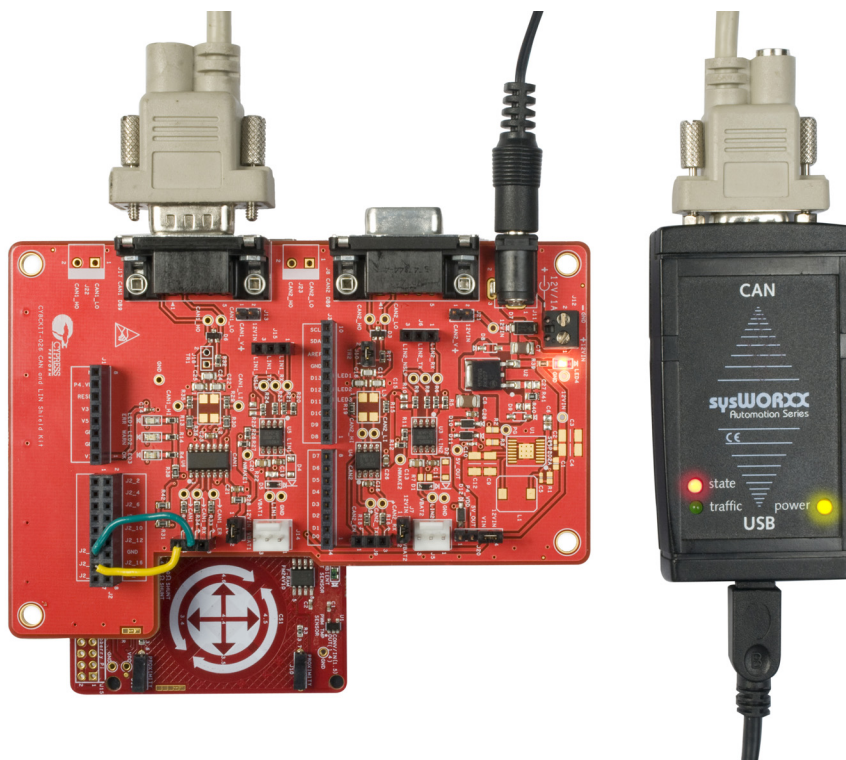
Figure 4-2. CAN Analyzer Connection to CY8CKIT-026's CAN1 Transceiver
