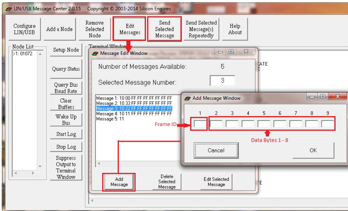
Figure 5-8. Adding and Sending Message using LIN Analyzer
