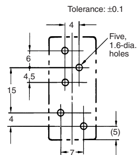
Mounting Holes
