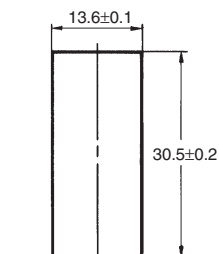
Panel Cutout
