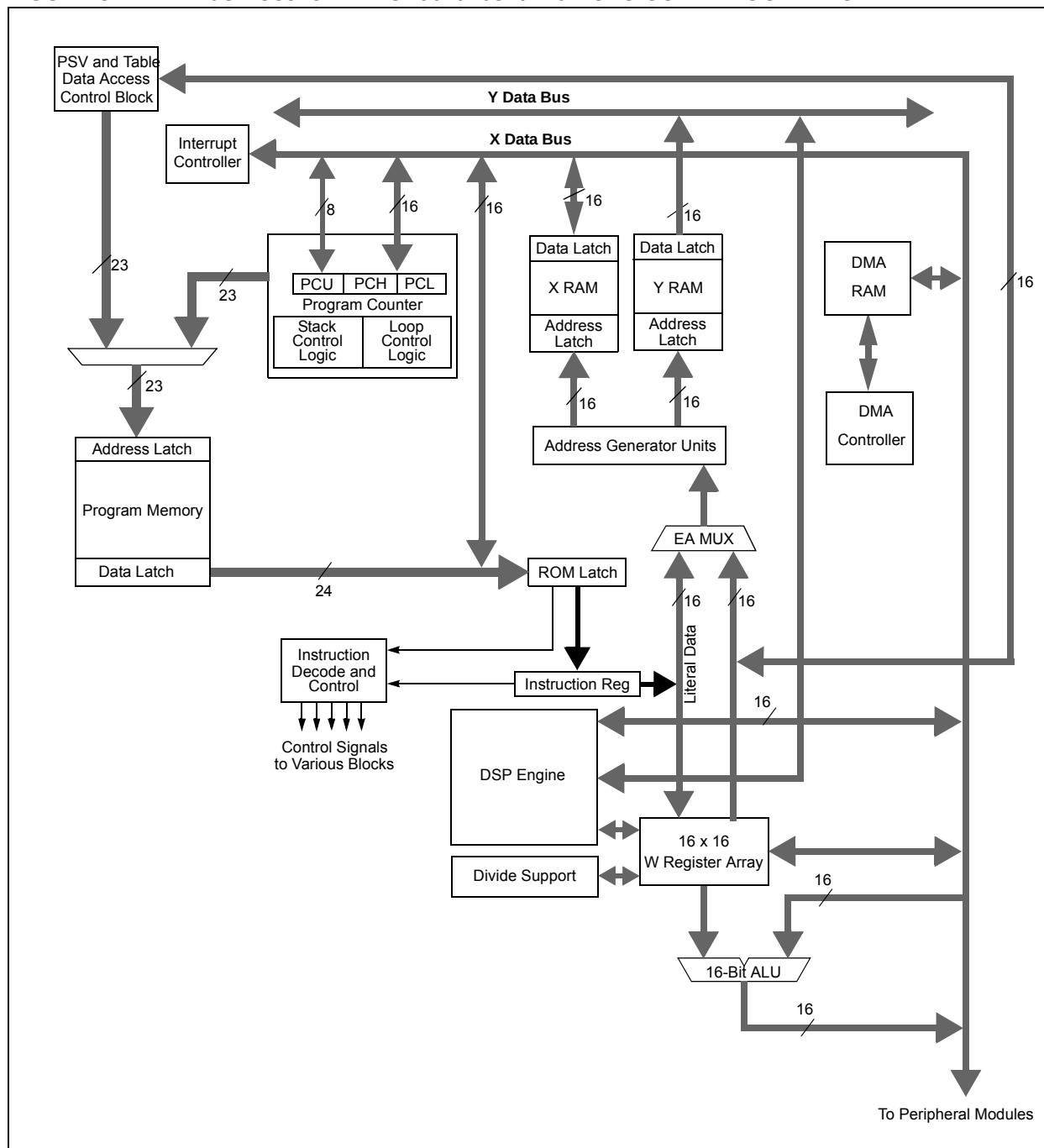
FIGURE 3-1: dsPIC33FJXXXMCX06A/X08A/X10A CPU CORE BLOCK DIAGRAM
