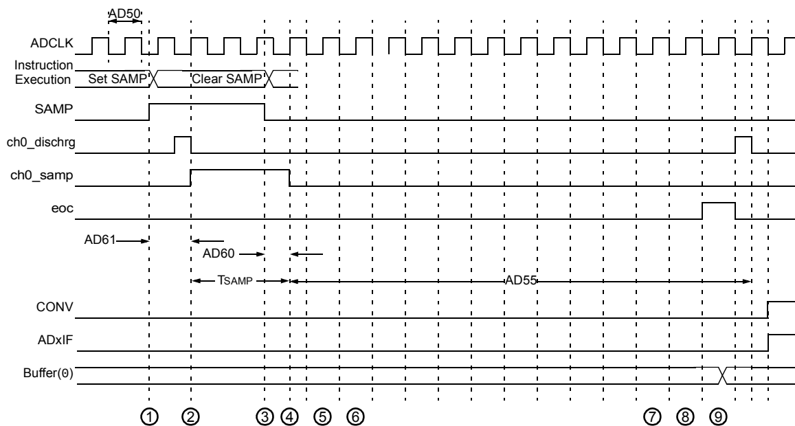
FIGURE 26-27: ADC CONVERSION (12-BIT MODE) TIMING CHARACTERISTICS (ASAM = 0, SSRC<2:0> = 000)
