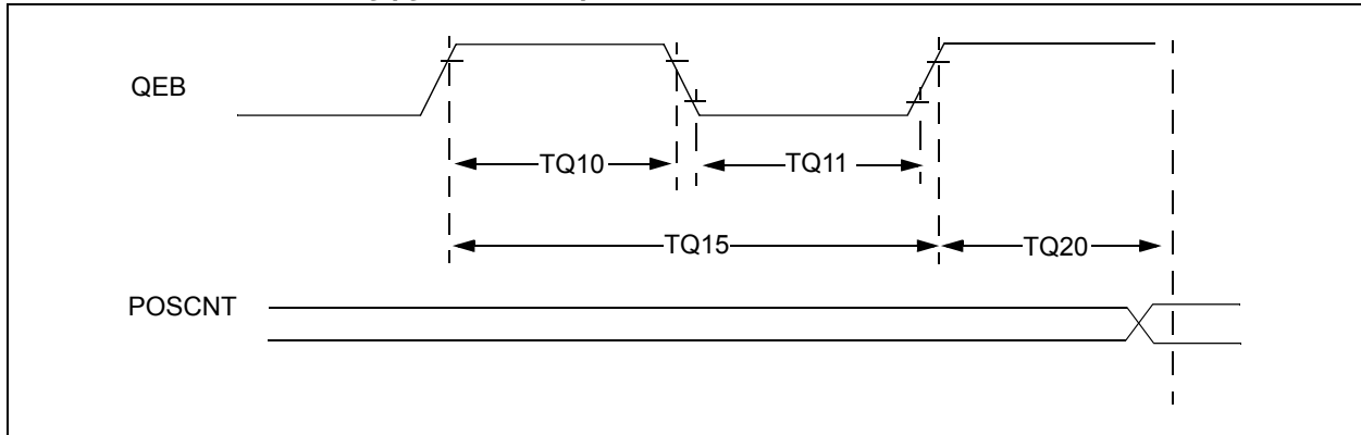
FIGURE 26-13: TIMERQ (QE1 MODULE) EXTERNAL CLOCK TIMING CHARACTERISTICS
