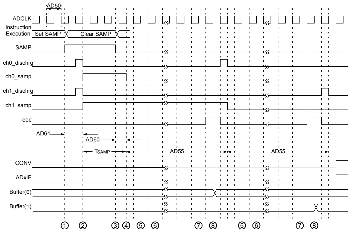
FIGURE 26-28: ADC CONVERSION (10-BIT MODE) TIMING CHARACTERISTICS (CHPS<1:0> = 01, SIMSAM = 0, ASAM = 0, SSR<2:0> = 000)
