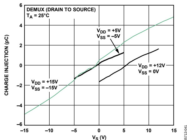
Figure 18. Drain-to-Source Charge Injection vs. Source Voltage
