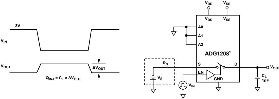
1 SIMILAR CONNECTION FOR ADG1209.
