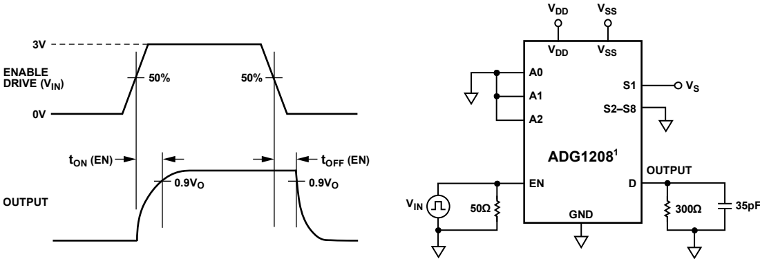
1 SIMILAR CONNECTION FOR ADG1209.
