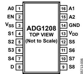
Figure 4. 16-Lead SOIC Pin Configuration (ADG1208)
