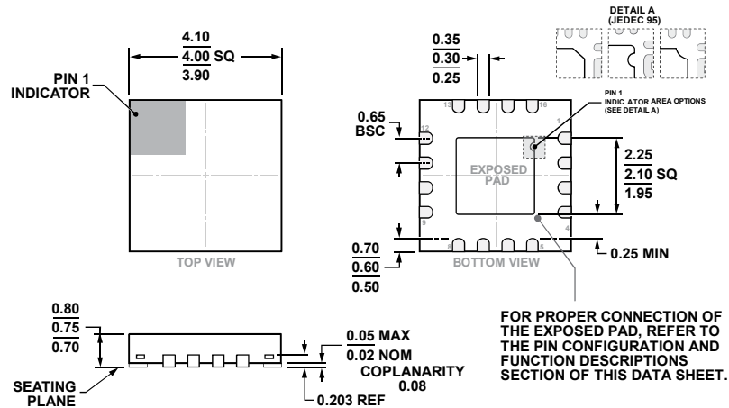
Figure 43. 16-Lead Lead Frame Chip Scale Package [LFCSP] 4 mm × 4 mm Body and 0.75 mm Package Height (CP-16-23) Dimensions shown in millimeters
