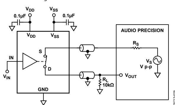
Figure 41. THD + N
