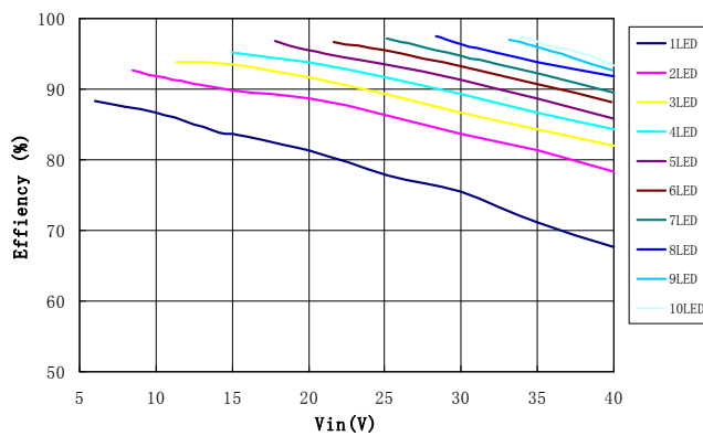
Efficiency vs. No. of LEDs L=47\mu\text{H} , R_s=0.33\Omega
