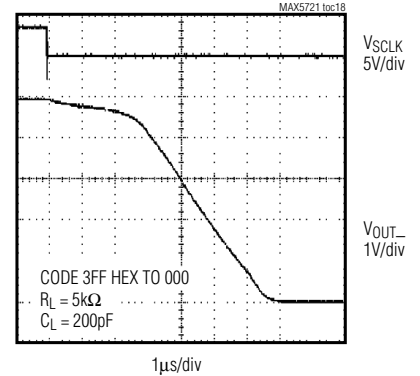
FULL-SCALE SETTLING TIME ( V_{DD} = +5\text{V} )
