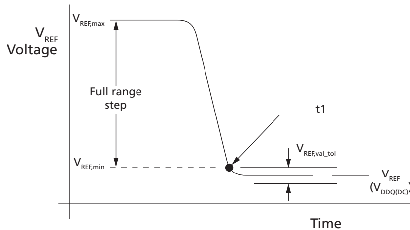
Figure 68: V_{\text{REF}} Full Step: From V_{\text{REF,max}} to V_{\text{REF,min}} Case
