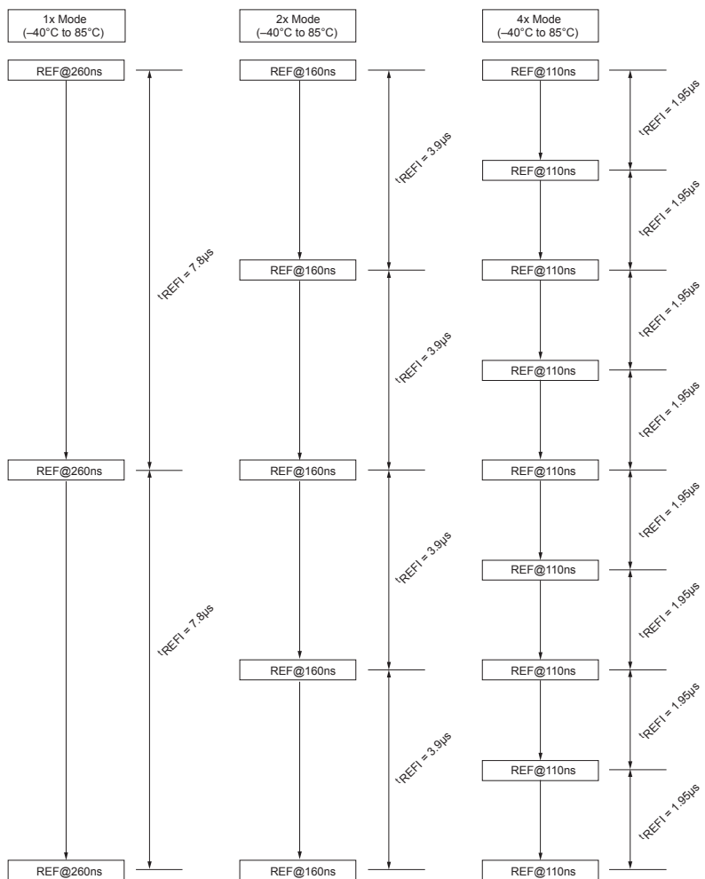
Normal Temperature Operation – -40^{\circ}\text{C} to 85^{\circ}\text{C}
