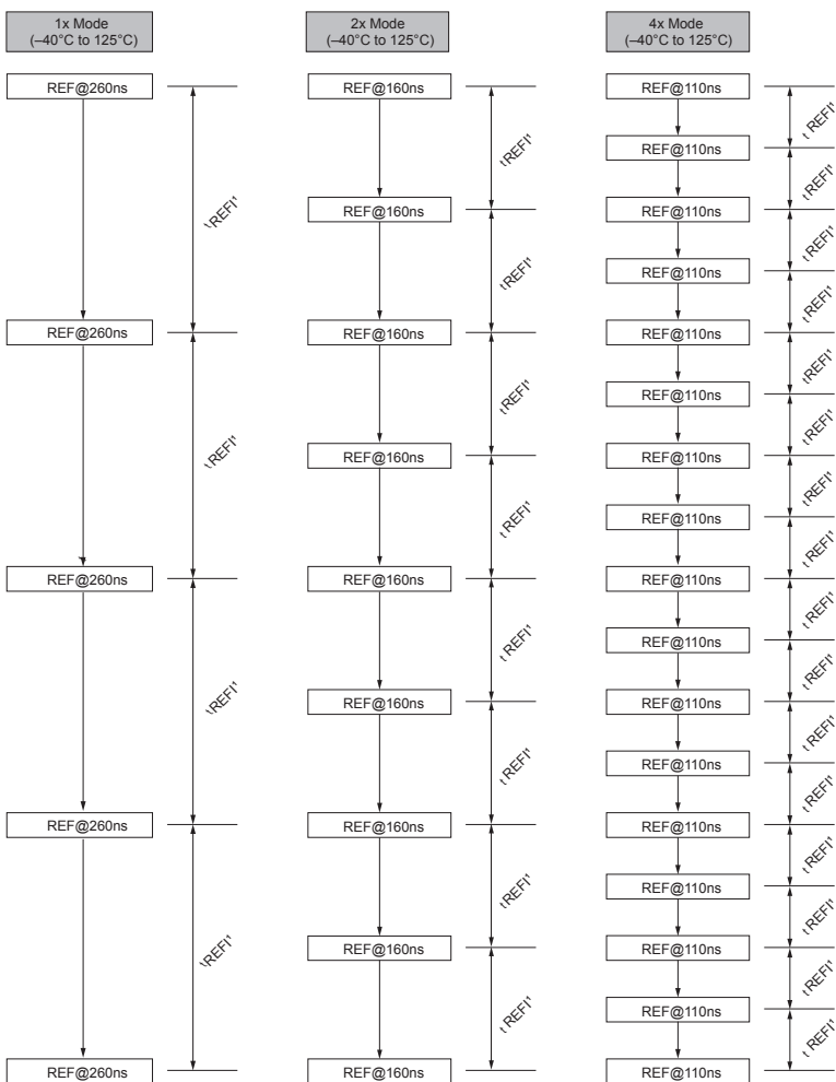
Extended Temperature Operation – –40°C to 125°C
