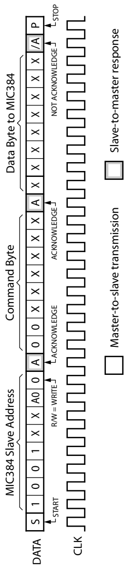
Figure 1. WRITE_BYTE Protocol
