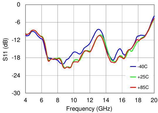
Average IRL vs. Temperature All phase states
