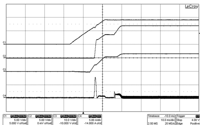
Figure 10. Start-up
