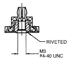
Press-In Bolt
