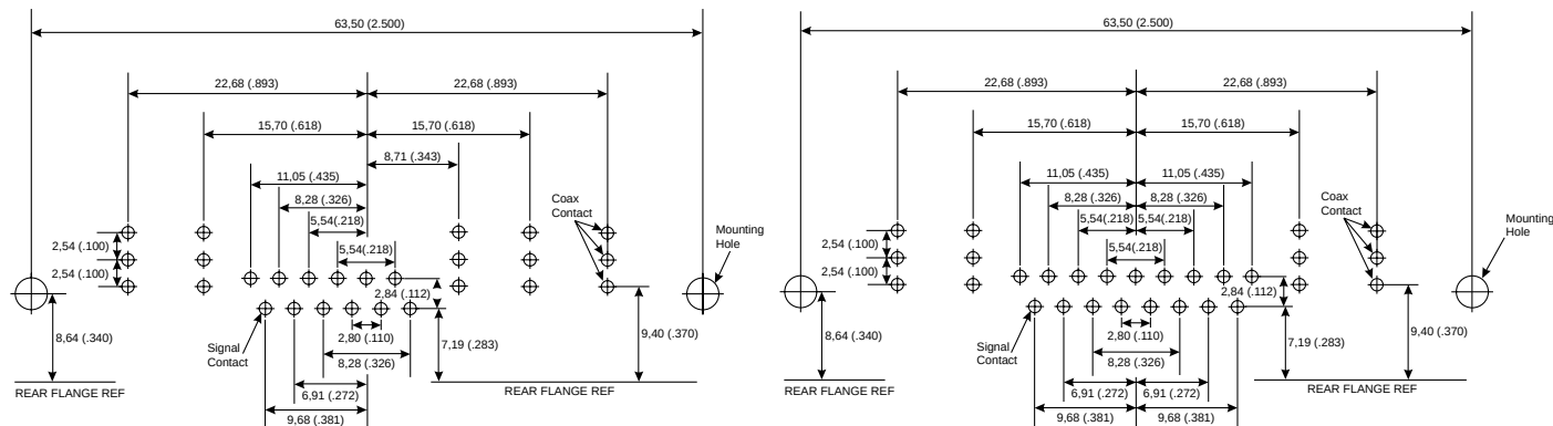
Shell Size Contact Arrangement No. of Size 20 Cavities No. of Size 8 Cavities C 17W5 12 #20 5 #8 Shell Size Contact Arrangement No. of Size 20 Cavities No. of Size 8 Cavities C 21WA4 17 #20 4 #8
