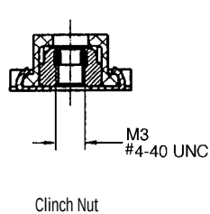
Clinch Nut
