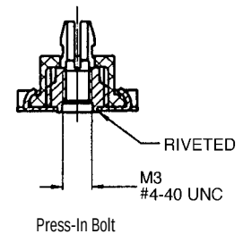
Press-In Bolt
