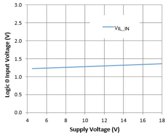
Figure 18. Logic 0 Input Voltage vs. Supply Voltage
