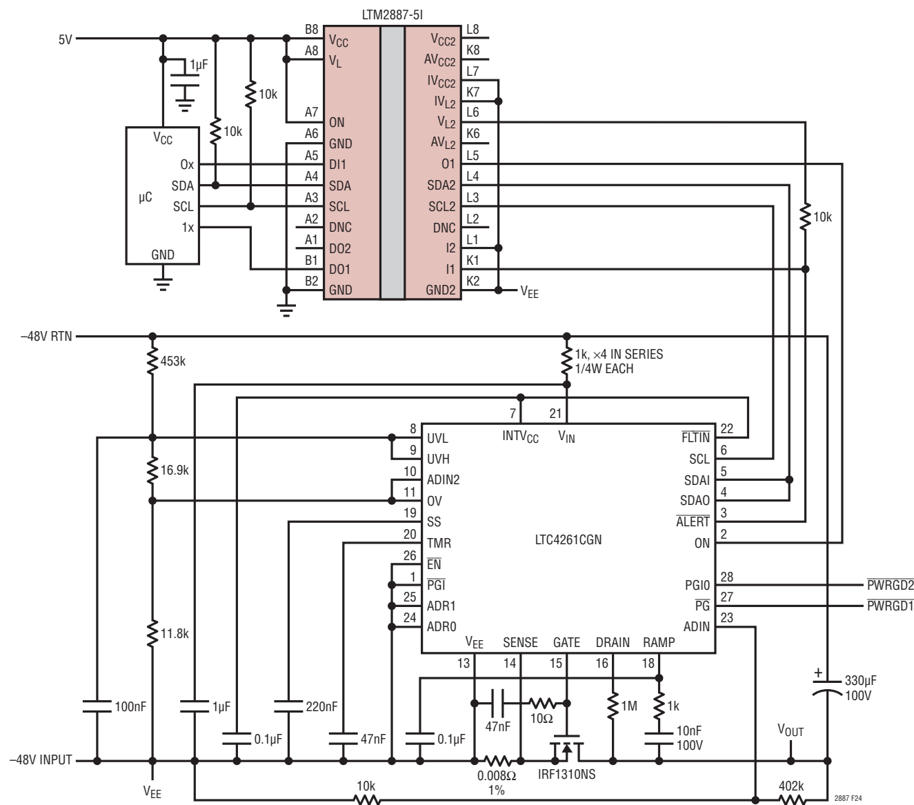
Figure 24. -48V, 200W Hot Swap Controller with Isolated I²C Interface
