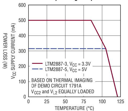
Derating for 125°C Maximum Internal Operating Temperature
