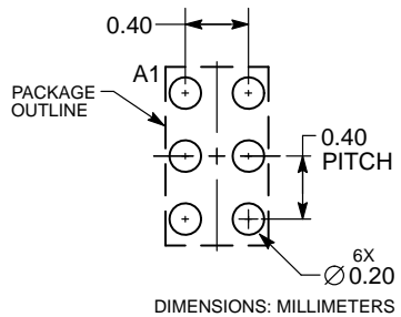
DIMENSIONS: MILLIMETERS
